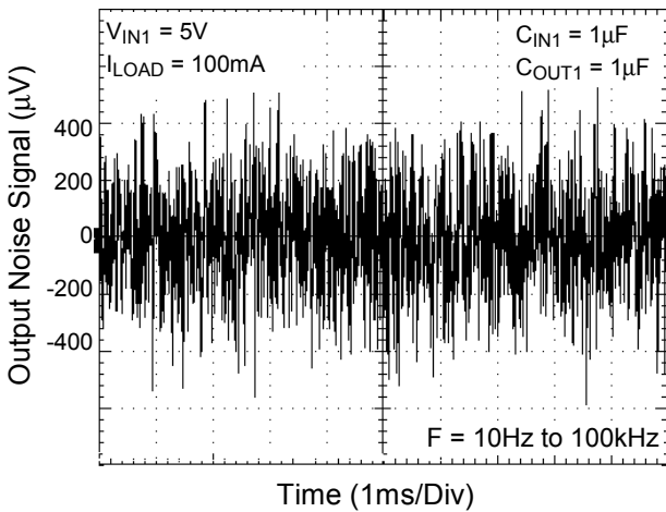
Output Noise
