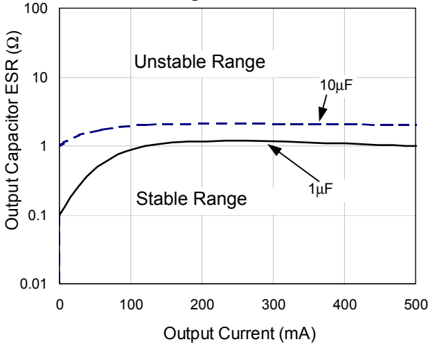
Range of Stable ESR
