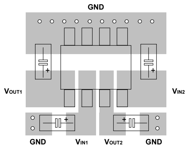
SOP-8 Board Layout
